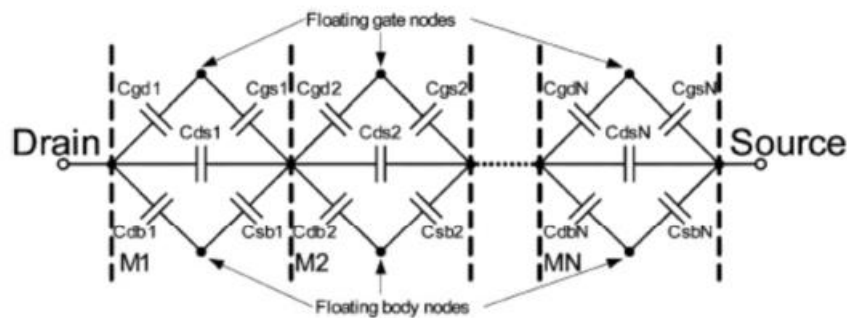
Fig. 5. Equivalent circuit of an N -series-connected transistor switch in the off state. (For the 20-finger 285\text{-}\mu\text{m} off-state transistor used: C_{gs} = 145\text{ fF} , C_{gd} = 144\text{ fF} , C_{db} = 2.6\text{ aF} , C_{sb} = 2.8\text{ aF} , C_{ds} = 15\text{ aF} ).
